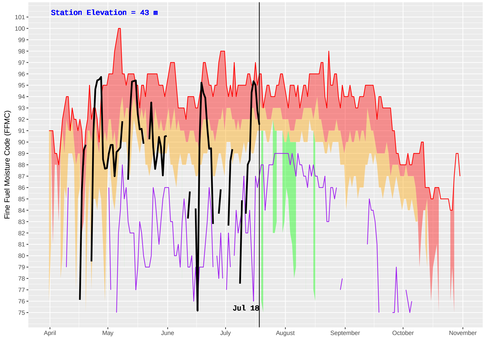
TOBA CAMP (75) : Historical (1970–2016) and Current (2018) Daily Fine Fuel Moisture Code (FFMC)
