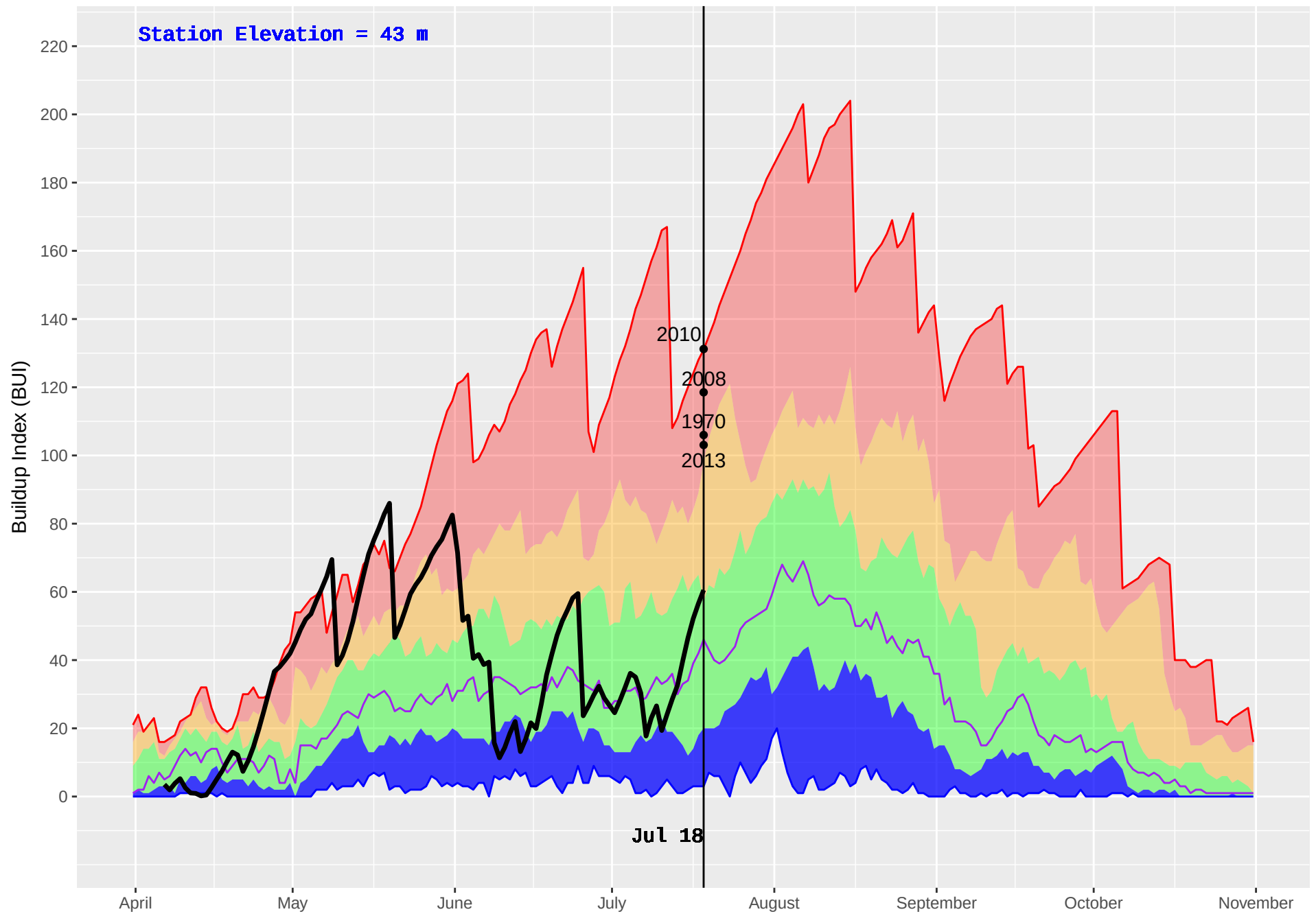
TOBA CAMP (75) : Historical (1970–2016) and Current (2018) Daily Buildup Index (BUI)
