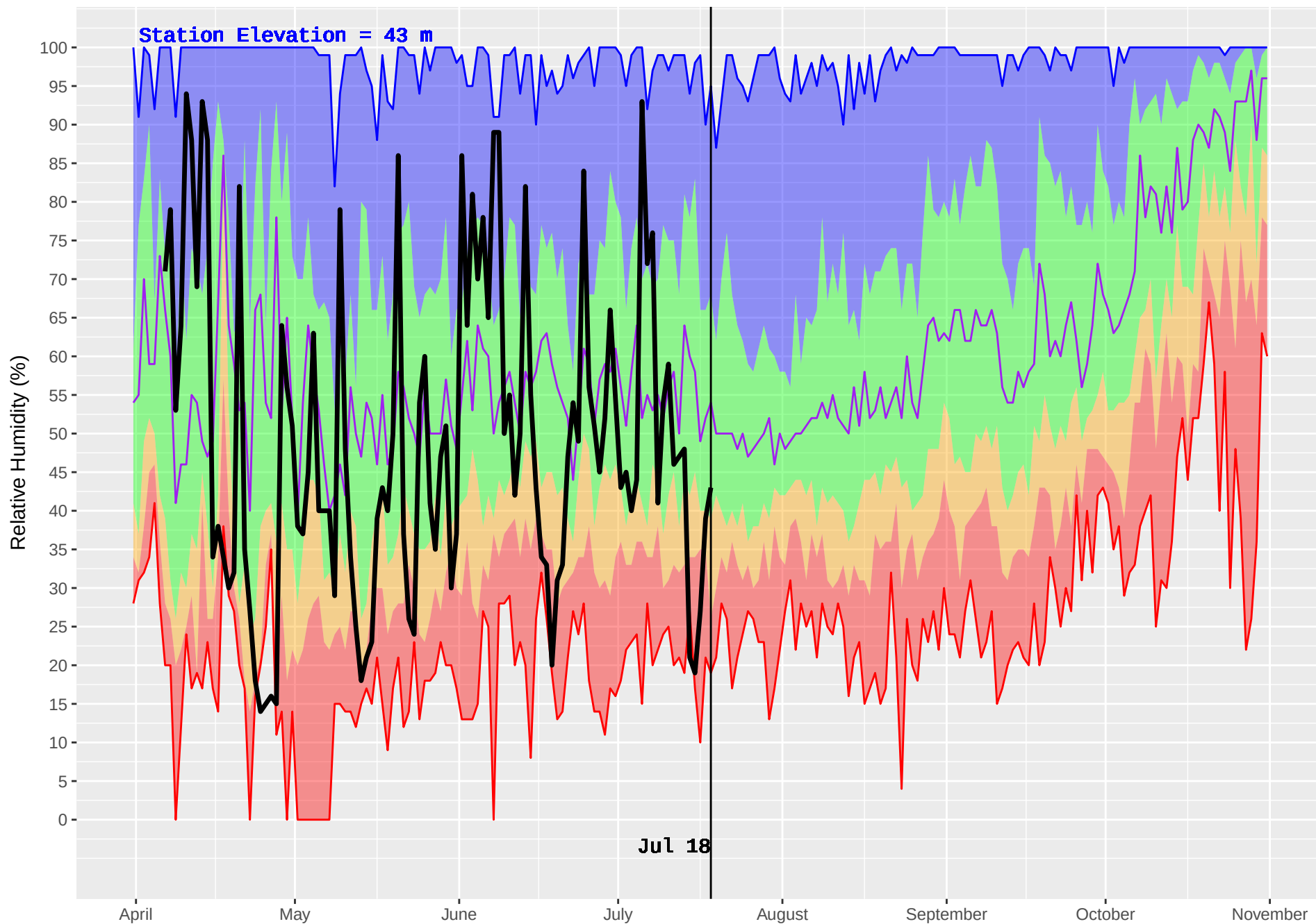
TOBA CAMP (75) : Historical (1970–2016) and Current (2018) Daily Relative Humidity
